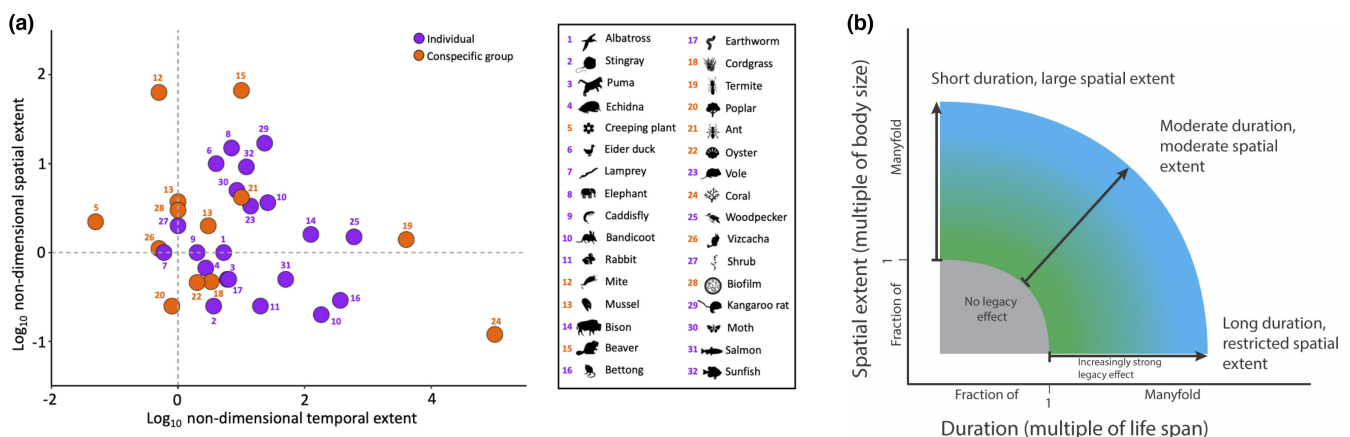
FIGURE 4 Non-dimensional framework for evaluating the strength of ecosystem engineering legacy effects. (a) Ecosystem engineering examples that illustrate the wide range of legacies documented in the literature, scaled by life span and body size of the engineer. Legacy effect is a function of structure duration (temporal extent relative to time of engineer occupation) and size (spatial extent relative to engineer body size). Living strategies of the engineer(s) may influence the relative importance of spatial versus temporal extent, as suggested by the differences in plotting positions of single individuals (purple) and conspecific groups (orange). We categorized each example as individual or group by taking cues from the language used by the author(s) of the original paper when the information was not explicitly stated; see Table 2 and Appendix A for additional information. (b) A general framework for relating legacy magnitude to the life span and body size of the engineer doing the work. Legacies fall along a gradient, where those that last as long or longer or are as large or larger than the engineer are stronger (blue), and those that are relatively brief or small are weaker (green) or negligible (grey).
