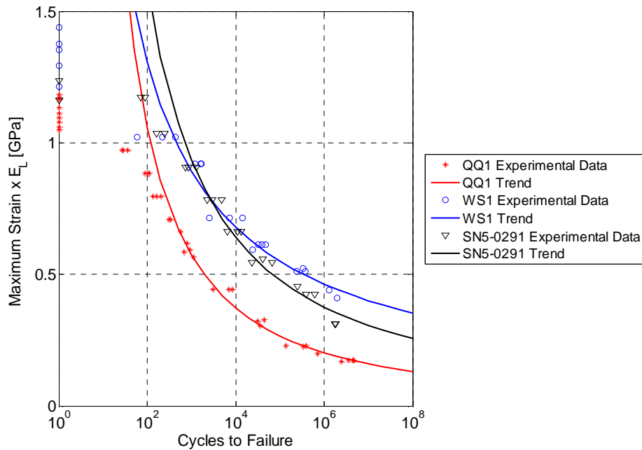
Figure 10. Tensile Fatigue Comparison of E-Glass/Epoxy Materials QQ1 and SN5-0291, and Windstrand/Epoxy Material WS1, R = 0.1 , Calculated 0^\circ Ply Stress ( E_L \cdot \text{Strain} ) vs. Cycles.
