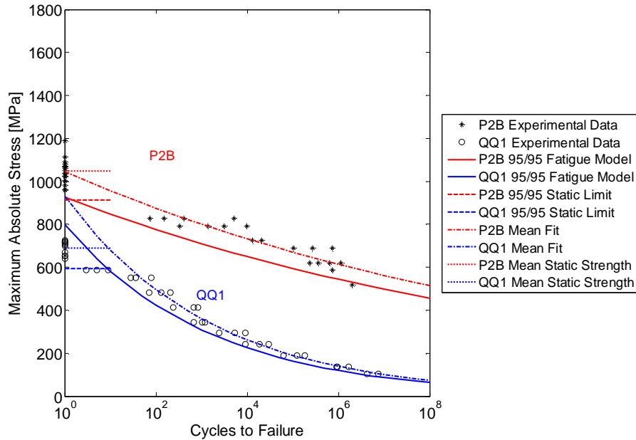
Figure 7(b). R = -1.
