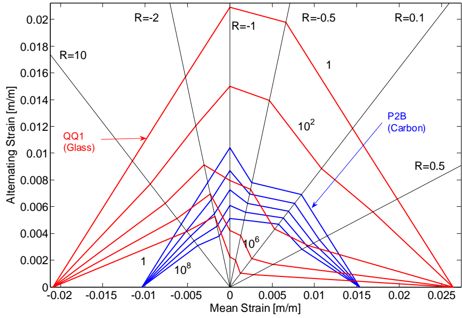
Figure 15. Comparison of Materials QQ1 (E-Glass) and P2B (Carbon Dominated), Strain Constant Life Diagram, Mean Strain S-N Model.
