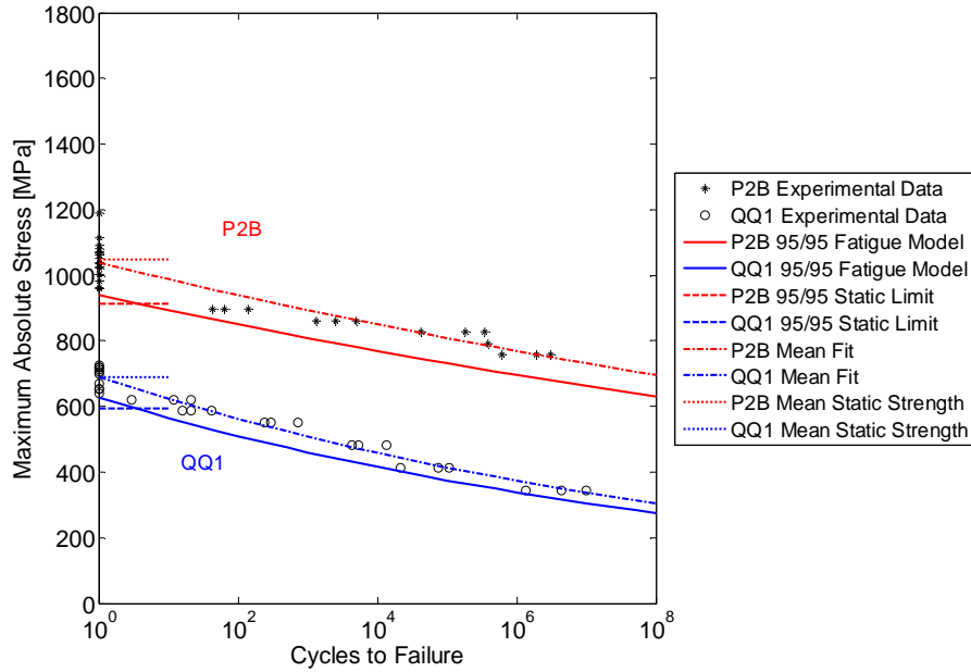
Figure 7(a). R = 10.
