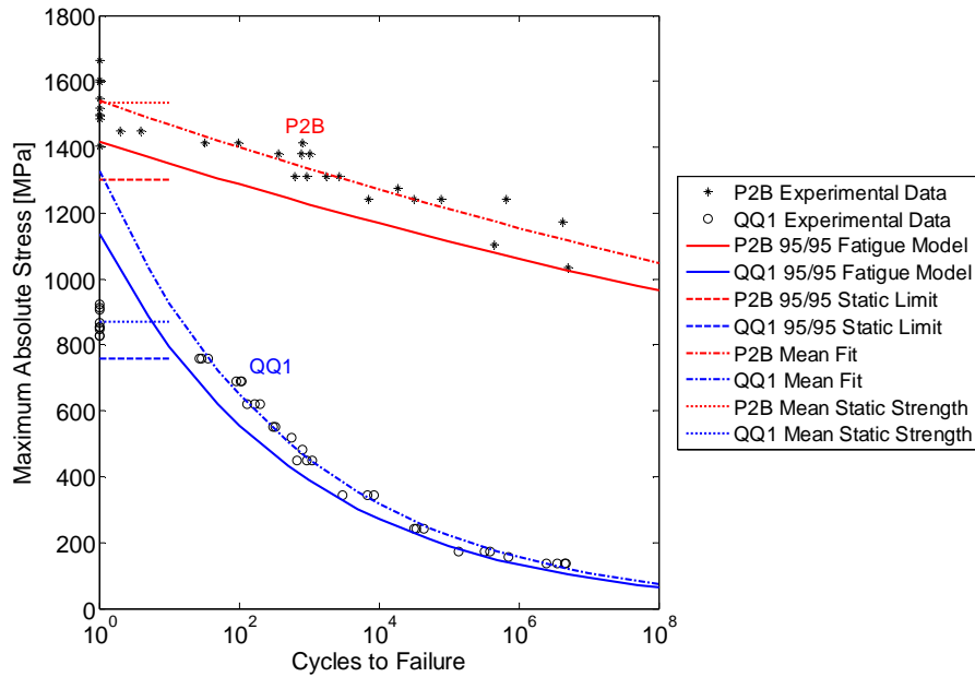
Figure 7(c). R = 0.1.
