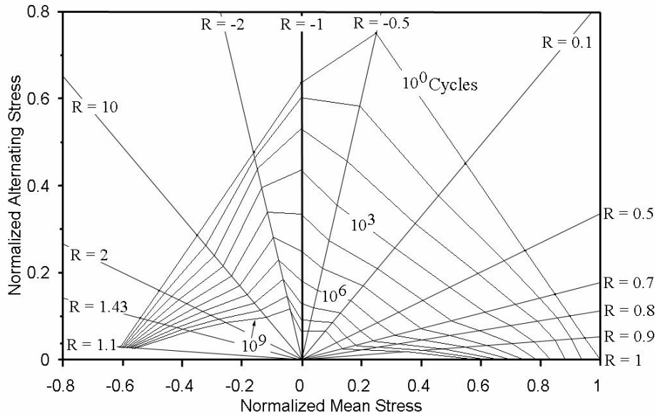
Figure 1. Constant life diagram for [90/0/\pm 45/0]_s E-glass/polyester laminate (0.36 fiber volume fraction) based on S-N data for 13 R-values, three-parameter Mean S-N model, axial ( 0^\circ ) load direction 5 (Normalized by the Static Tensile Strength).
