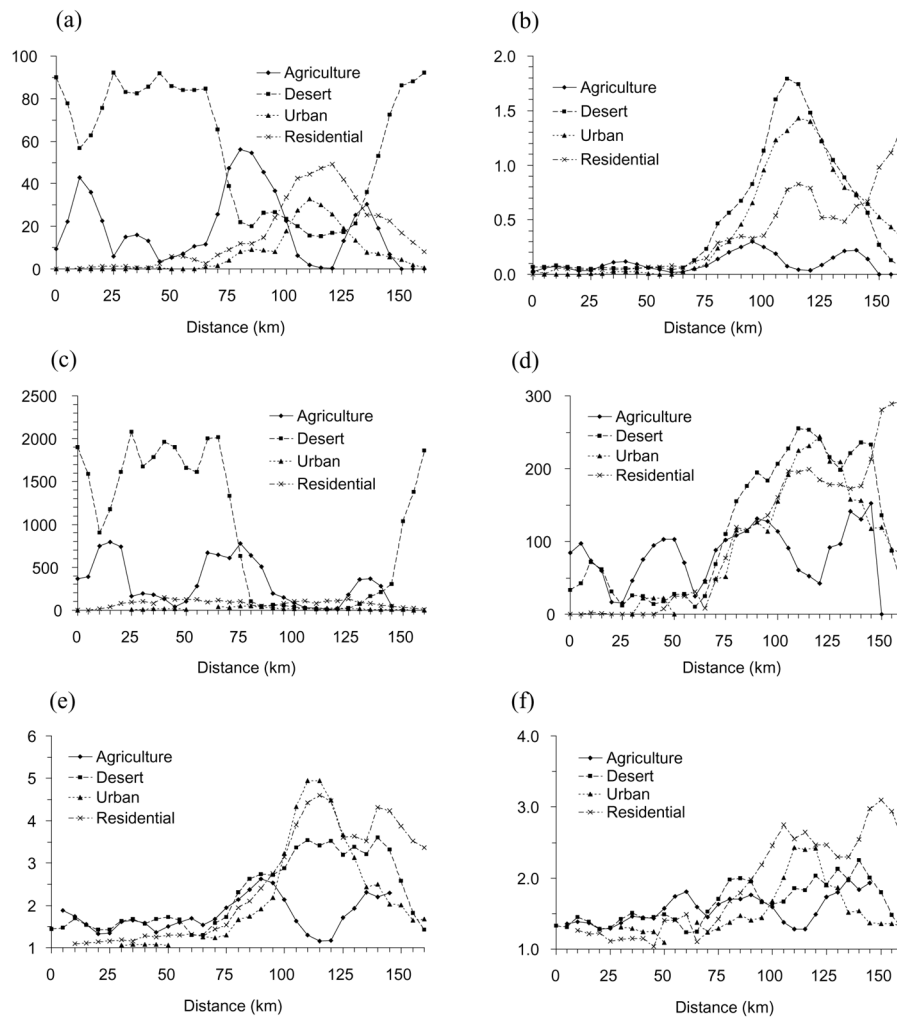
Figure 3. Changes in landscape pattern along the transect by patch type: (a) patch type percent cover, (b) patch density, (c) mean patch size, (d) patch size coefficient of variation, (e) landscape shape index, and (f) area-weighted mean shape index. The values were averages obtained using a 3 \times 3 overlapping moving window. See text for explanations.
