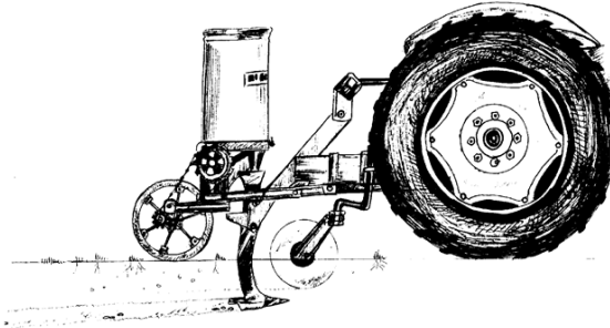
Fig. 9. A pocket gopher burrow builder. The burrow builder meters out grain bait into an artificial burrow. Pocket gophers enter the artificial burrow where it intersects the natural burrow and find the bait.
