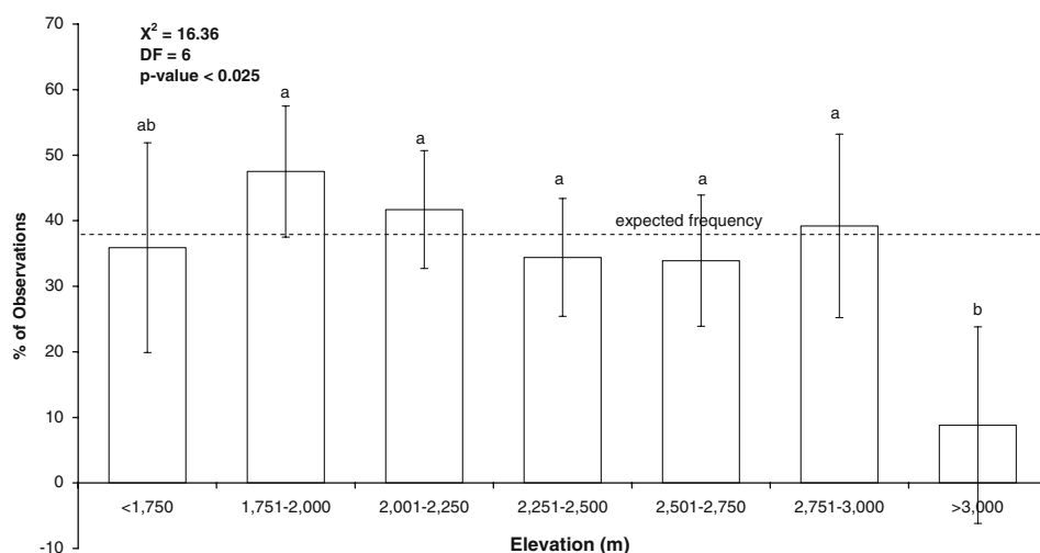
Figure 4. Frequency of conifer cover increase by elevation class. Dashed line represents the expected frequency. The Chi-square statistic is reported at the top left along with its corresponding p-value. Frequencies are shown with Bonferonni corrected 95% confidence intervals. Frequencies with the same letter do not differ significantly.
