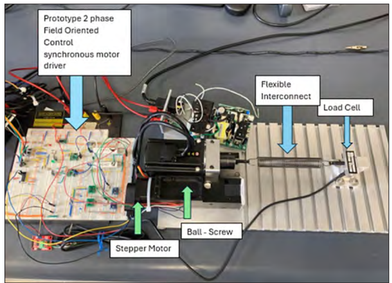
Figure 2. MSU is developing a synchronous motor driver to operate as a hybrid brushless DC motor (torque proportional to current) to drive a conventional stepper motor.
