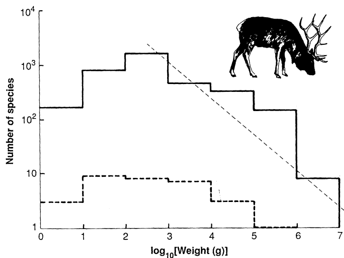
Fig. 2. The numbers of species, S , of all terrestrial mammals (solid histogram) and of British mammals (dashed histogram), excluding bats, are shown distributed according to mass categories (mass expressed in grams) (18, 19). Note the doubly logarithmic scale. The thin dashed line illustrates the shape of the relation S \sim L^{-2} , where L is the characteristic length (20).
